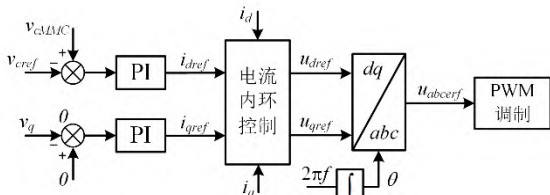
图 2 辅助 VSC 换流器稳态运行阶段控制框图 Fig. 2 The steady-state operation control diagram for the VSC auxiliary converter
