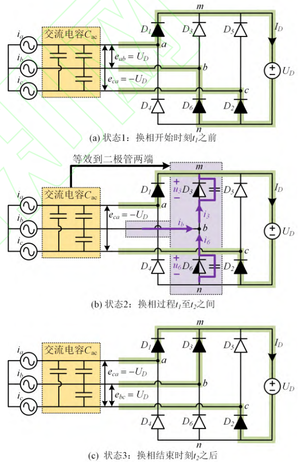
图 5 二极管 D_6 向 D_3 换相及换相前后的实际导通电路 Fig. 5 The actual conduction circuit before, during, and after the commutation process of diode D_6 to D_3
