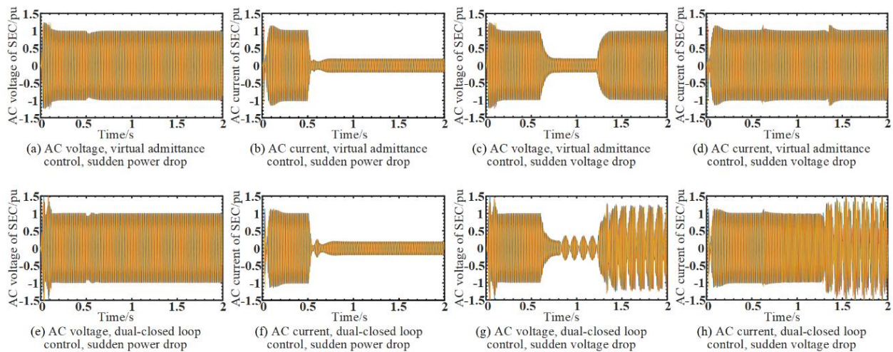
Fig. 7. Simulation result of different control strategies under various operating conditions
